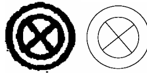
Circle vectorization
