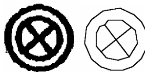
Lines vectorization
